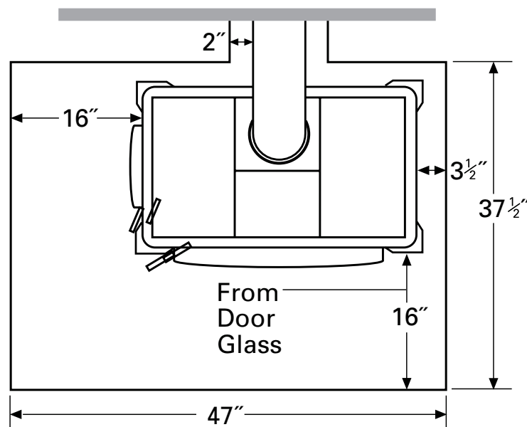
Minimum Hearthpad Dimensions
